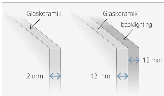
Cross section of the rear wall structure
